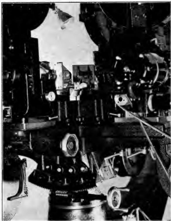
FIG. 2. Partial side view, showing vertical tilt device; also focusing handwheel in center. Rear view of mirror and adjustment screws.
